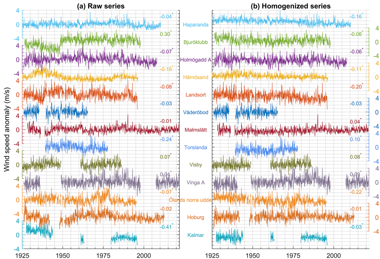
Figure 5. Comparison of (a) raw and (b) homogenized wind speed anomaly series rescued at the 13 stations in Sweden. The long-term trends (in \text{m s}^{-1} per decade) are shown on the right, with * indicating a significance level of 0.05.
