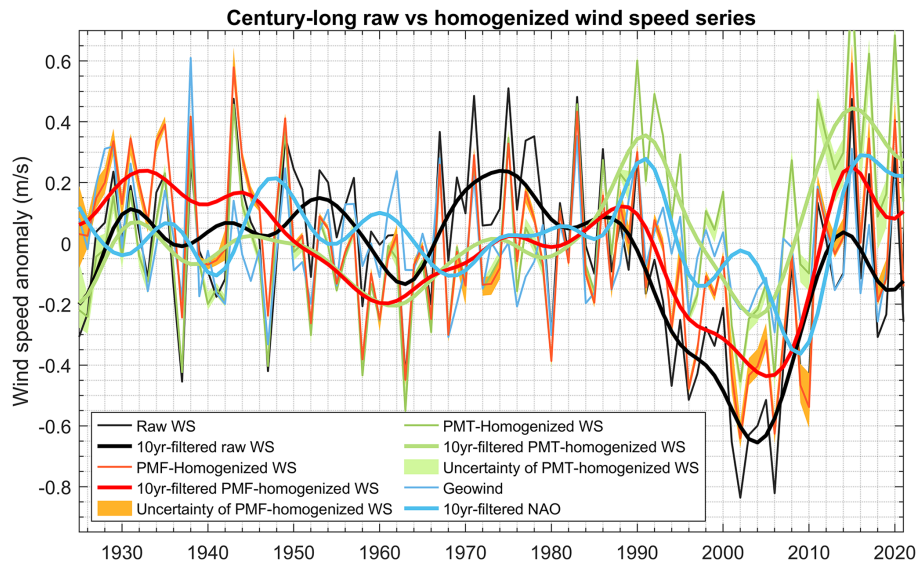
Figure 6. The averaged wind speed anomaly series at the 13 stations from raw and homogenized data (in black, red or green lines). The uncertainty of the homogenized data with CERA-20C 10-member ensembles as the reference series is shown in brown or green shading. The 10-year low-pass-filtered series of raw data, homogenized data, and scaled North Atlantic Oscillation (NAO) are shown by thick lines. Geowind series is also shown to depict the signal of internal climate variability (in blue line). For comparison, the PMF and PMT tests were applied to detect change points during the homogenization.
