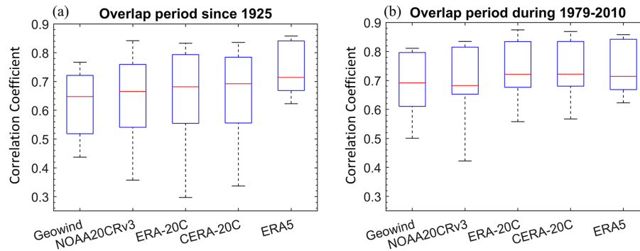
Figure 2. Box plot for correlation coefficients of monthly wind speed anomaly series between the rescued data at the 13 stations and the geowind or reanalysis data at the collocated grids (a) during the paired overlap periods since 1925 and (b) during the all-datasets overlap period, 1979–2010.
