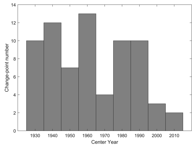
Figure 3. Histogram of the years of the detected change points. Bars are grouped every 10 years.
