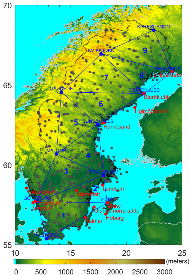
Figure 1. Map of the 13 stations (red points), with century-long rescued wind speed series and nine pressure triangles (blue lines) used to calculate the geowind data since 1925. Other weather stations in Sweden, installed to measure routine meteorological variables since 1956–1978s, are shown as grey points. Shading is the topography (in meters) from the global 30 arcsec elevation dataset (GTOPO30).
