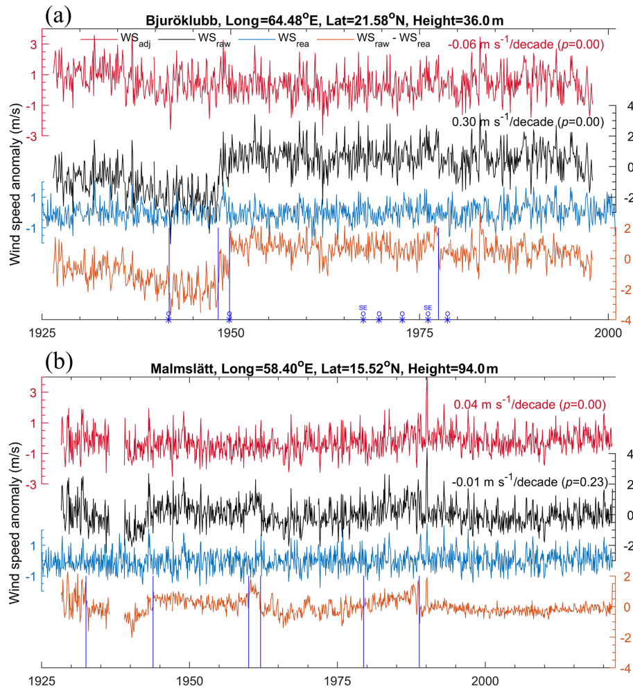
Figure 4. Two examples to illustrate the homogenization process and result. Black, blue, and red lines are raw ( WS_{\text{raw}} ), reanalysis ( WS_{\text{rea}} ), and adjusted ( WS_{\text{adj}} ) series of monthly wind speed anomaly, respectively. The brown line is the residual (raw series minus reanalysis series: WS_{\text{raw}} - WS_{\text{rea}} , calculated by linear regression) used for removing the natural climate variability from the raw series, which then amplifies spurious discontinuities during the homogenization. The reanalysis reference series was estimated from the climate reanalysis CERA-20C (1925–2010) and extended by the latest ERA5 (2011–2021). Blue vertical lines show the detected change-point dates, and blue asterisks show the changes in the events recorded in the collected metadata; for example, “O” represents a change in the observatory and “SE” shows changes in the surrounding environments. The long-term trends in wind speed are shown in the top right.
