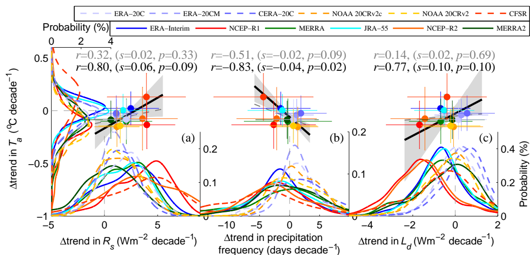
Figure 8. Spatial associations of the simulated biases in the trend in surface air temperature ( T_a ) versus three relevant parameters among the 12 reanalysis products (solid lines indicate the NWP-like reanalyses, and dashed lines indicate the climate reanalyses). The probability density functions (unit: %) of these biases in the trends are estimated from approximately 700\ 1^\circ \times 1^\circ grid cells that cover China. The median values (coloured dots with error bars of spatial standard deviations) of the biases in the trends in T_a (unit: ^\circ\text{C decade}^{-1} ) in the 12 reanalyses are regressed onto those of (a) the surface incident solar radiation ( R_s , unit: \text{W m}^{-2} \text{ decade}^{-1} ), (b) precipitation frequency (unit: \text{days decade}^{-1} ) and (c) the surface downward longwave radiation ( L_d , unit: \text{W m}^{-2} \text{ decade}^{-1} ) using the ordinary least-squares method (OLS, denoted by the dashed grey lines) and the weighted total least-squares method (WTLS, denoted by the solid black lines). The 5–95% confidence intervals of the regressed slopes obtained using WTLS are shown as shading. The regressed correlations and slopes are shown as grey and black text, respectively.
