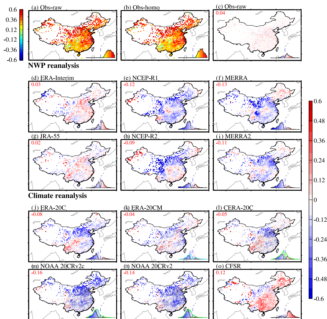
Figure 5. (a, b) The observed trends in surface air temperature ( T_a , unit: ^{\circ}\text{C decade}^{-1} ) and the simulated biases in the trends in T_a (unit: ^{\circ}\text{C decade}^{-1} ) during the period of 1979–2010 from (c) raw observations and (d–o) the 12 reanalysis products over China with respect to the homogenized observations. The squares denote the original homogeneous time series, and the dots denote the adjusted homogeneous time series. The probability distribution functions of all of the biases in the trends are shown as coloured histograms, and the black stars are integrated from the trend biases with a significance level of 0.05 (based on two-tailed Student's t tests). The cyan and green stars in (k–n) represent estimates of the biases in the trends outside the ensemble ranges whose locations are denoted by the black dots shown in (k–n).
