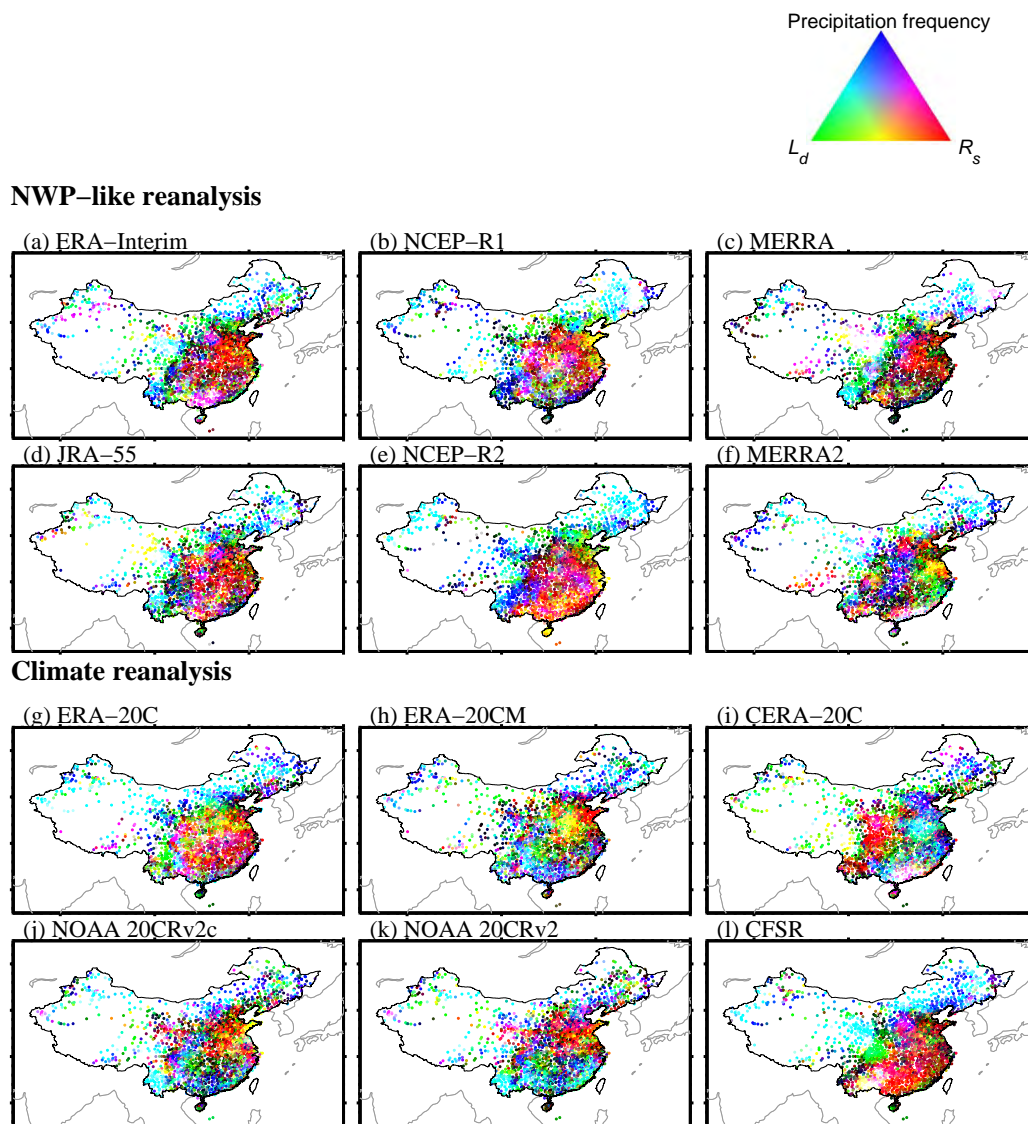
Figure 6. Composite map of the contributions (unit: ^{\circ}\text{C decade}^{-1} ) of the biases in the trends in three relevant parameters, surface incident solar radiation ( R_s , in red), surface downward longwave radiation ( L_d , in green) and precipitation frequency (in blue) to the biases in the trends in surface air temperature ( T_a ) during the study period of 1979–2010, as estimated using the 12 reanalysis products over China.
