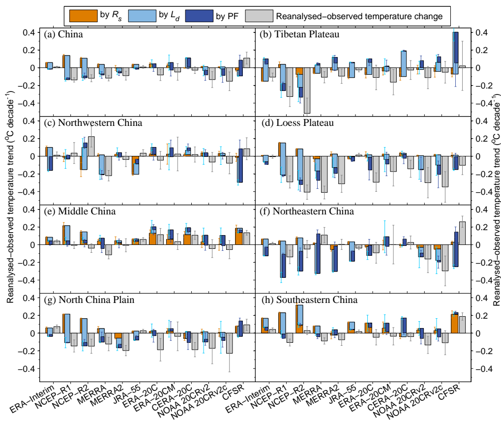
Figure 7. Contributions (unit: ^{\circ}\text{C decade}^{-1} ) of the biases in the trends in surface air temperatures ( T_a ) from three relevant parameters, surface incident solar radiation ( R_s , in brown), surface downward longwave radiation ( L_d , in light blue) and precipitation frequency (PF, in deep blue), during the study period of 1979–2010 from the 12 reanalysis products over China and its seven subregions.
